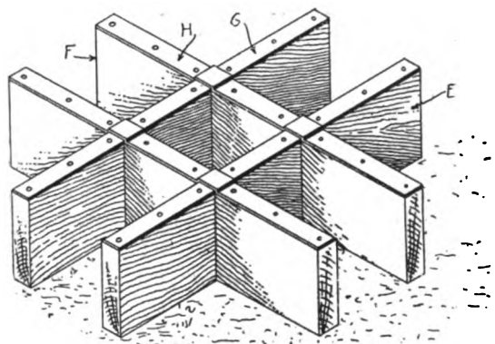
Fig. 1—The wooden wheel block and showing method utilized in fastening the strap irons
